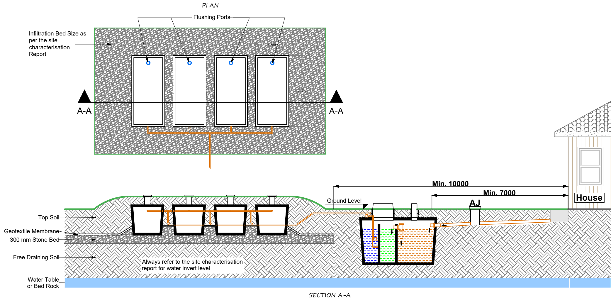
SECTION A-A StreamClear Modules 12PE
